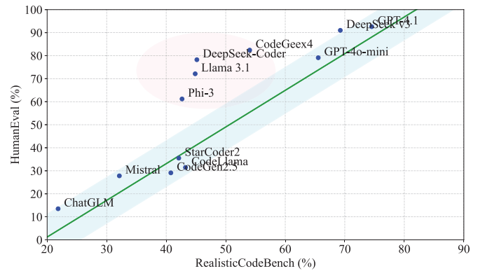
Fig. 3: The performance comparison of pass@1 for 12 LLMs between HumanEval and RealisticCodeBench (Python)
